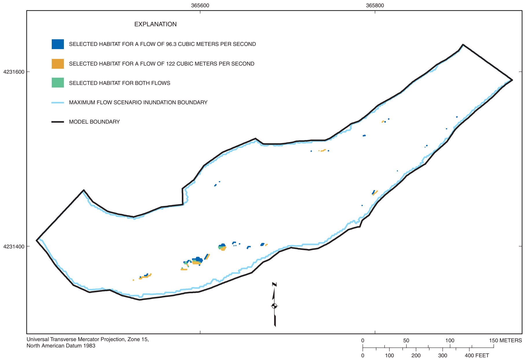
Figure 4-92. Selected habitat area distribution for habitat category 22 (channel catfish) at flows of 96.3 and 122 cubic meters per second at Marais des Cygnes River site MDC2.
